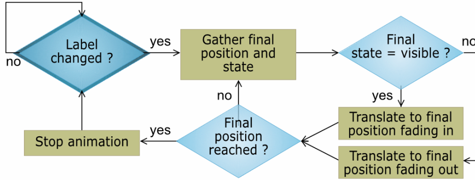
Figure 2: Flowchart of the described event handling. Starting point is the marked state in the upper left.
