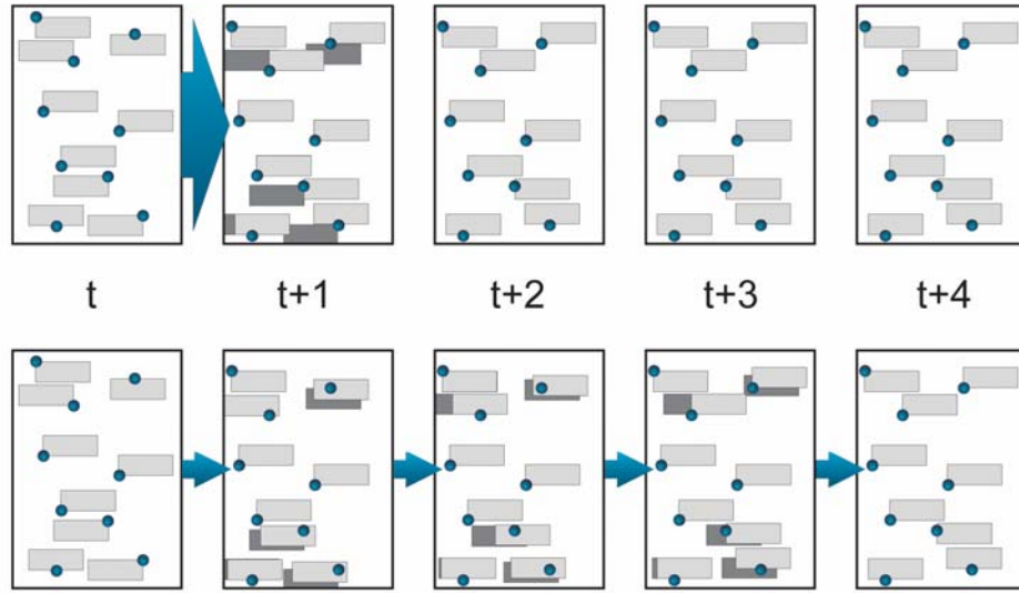
Figure 1: The proposed floating labels method. The upper row demonstrates rapid changes, while losing frame-to-frame coherence (dark grey: previous position, light grey: current position). Within the lower row floating labels are used, to spread instantaneous changes smoothly across several frames. Thus, the visual tracking of label positions is improved. Please take note of the accompanying video, demonstrating the technique more clearly.
